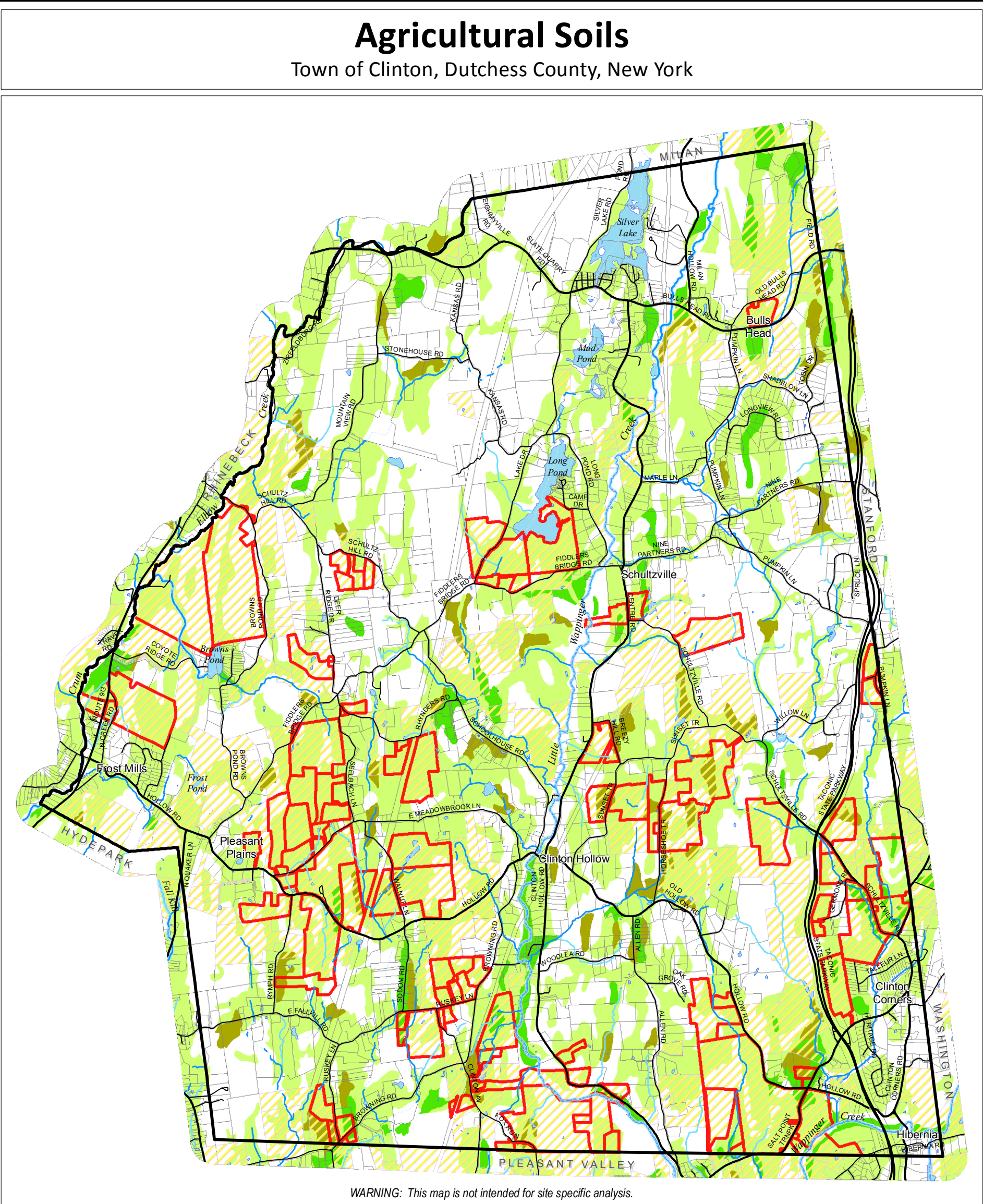
Figure 3.5 - Agricultural Soils Map
